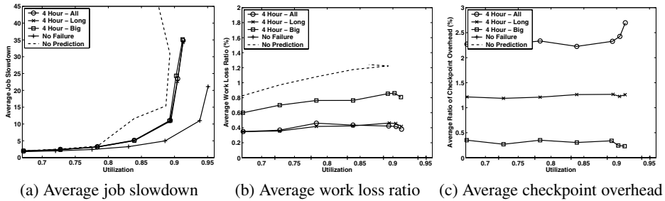
Fig. 9. Comparing three heuristics using four-hour buckets for iid failures ( \beta=0.85 ; W=2 ; \alpha=0.01 ; r=2 minutes).
