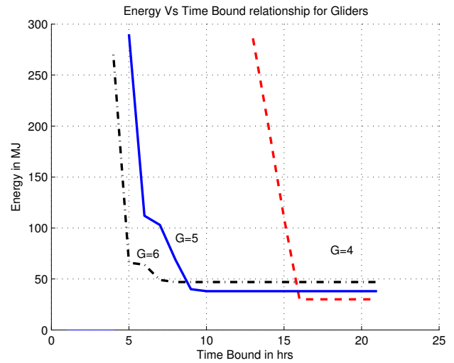
Figure 8: Relationship between the energy in MJ of gliders vs. the time bound for the mission \delta .
