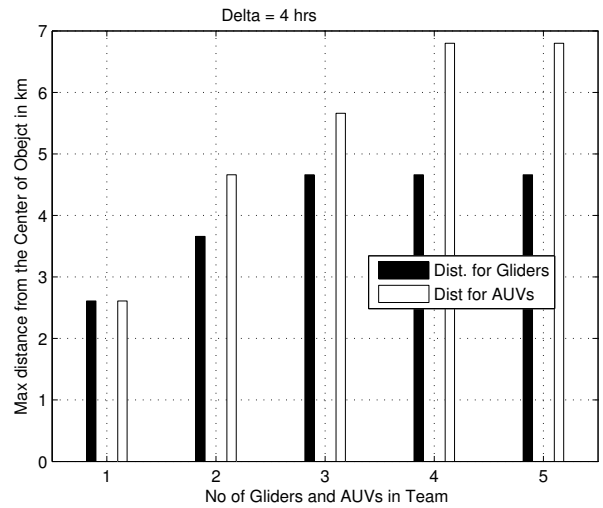
Figure 15: Maximum distance in km from which the gliders and AUVs are selected in the team against the team size when \delta is 4 hr.
