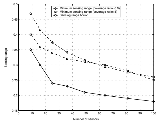
Figure 7: Theoretical and experimental sensing range
