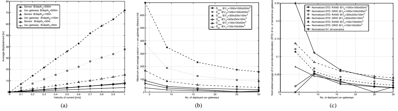
Figure 4: (a): Average horizontal displacement of sensors and uw-gateways vs. current velocity (for three different depths); (b): Maximum and average sensor-gateway distance vs. no. of deployed gateways (in three different volumes, and with v_c^{max} = 1 m/s); (c): Normalized average and standard deviation of no. of sensors per uw-gateway vs. no. of deployed gateways (for grid and random deployment strategies, in three different volumes, and with v_c^{max} = 1 m/s)
