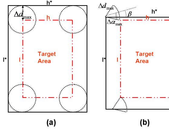
Figure 5: Deployment surface area for unknown (a) and known (b) current direction \beta , given a bottom target area l \times h
