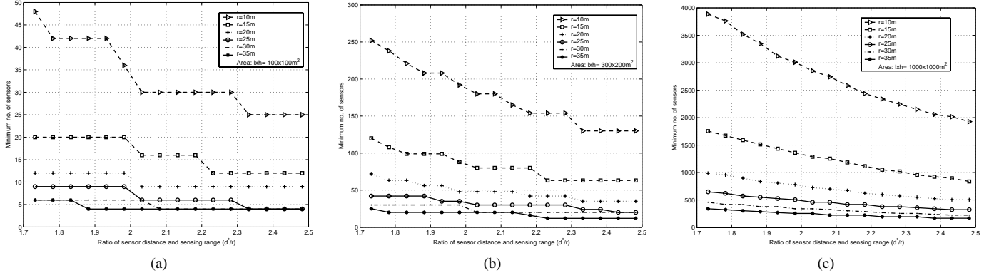
Figure 3: Minimum no. of sensors in triangular-grid deployment vs. sensor distance over sensing range. (a): A_1 = 100 \times 100 \text{ m}^2 ; (b): A_2 = 300 \times 200 \text{ m}^2 ; (c): A_3 = 1000 \times 1000 \text{ m}^2
