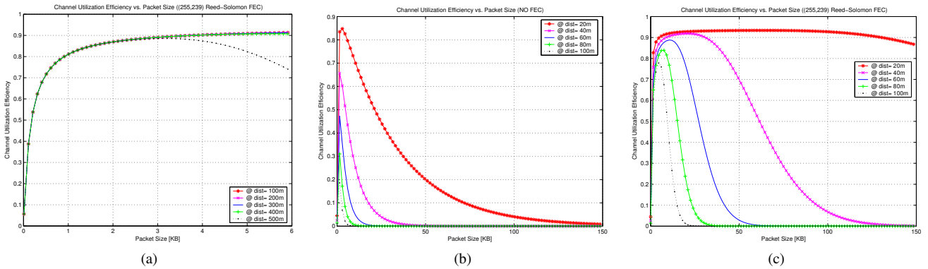
Figure 3: Terrestrial channel efficiency vs. packet size with Reed-Solomon FEC (a). Underwater channel utilization efficiency vs. packet size for different distances (20m-100m) without (b) and with Reed-Solomon FEC (c)
