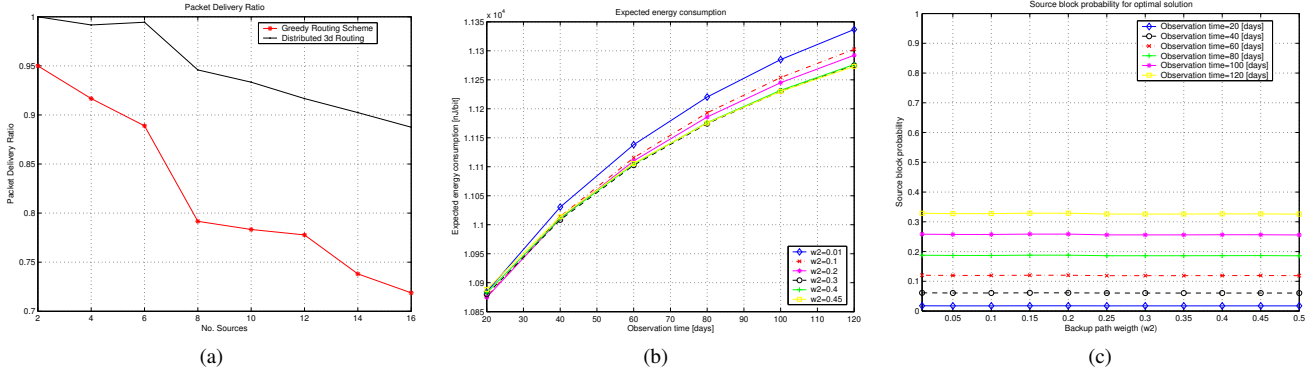
Figure 4: Packet delivery ratio for a greedy routing scheme and the distributed 3D routing (a). Expected energy consumption for primary and backup paths (b) and source block probability (c) for the centralized 3D routing
