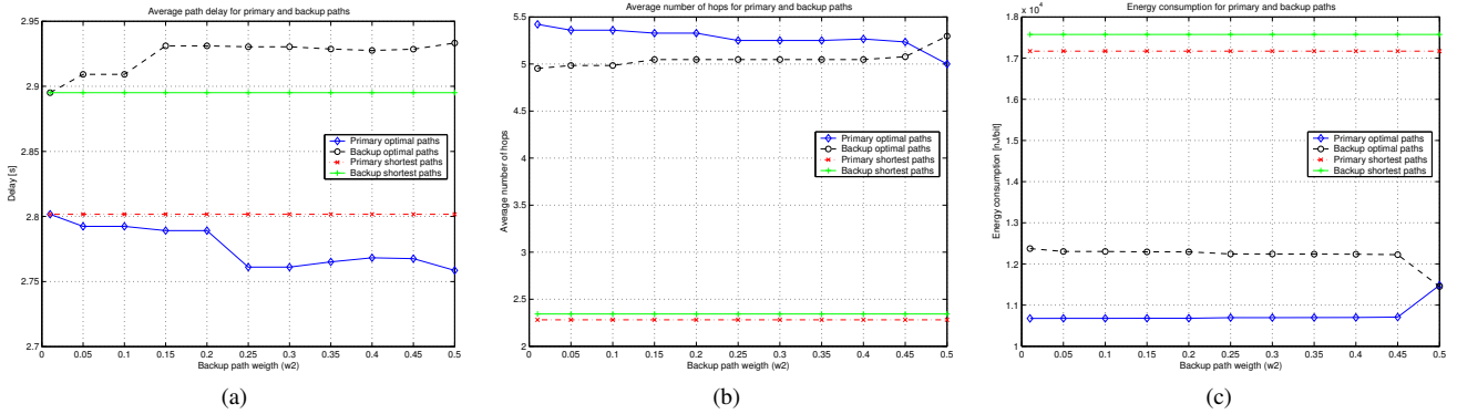
Figure 5: Comparison of average path delay (a) and average number of hops (b) for primary and backup paths (optimal and shortest path). Energy consumption for primary and backup path (optimal and minimum-hop path) (c)
