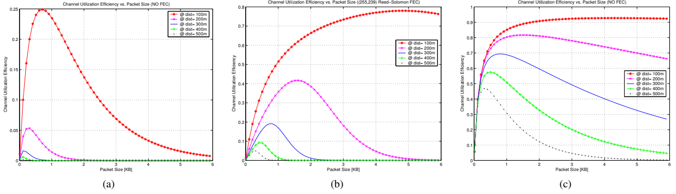
Figure 2: Underwater channel efficiency vs. packet size for different distances (100m-500m) without (a) and with Reed-Solomon FEC (b). Terrestrial channel efficiency vs. packet size without Reed-Solomon FEC (c)
