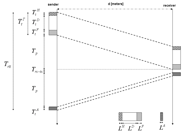
Figure 1: Underwater channel utilization efficiency
