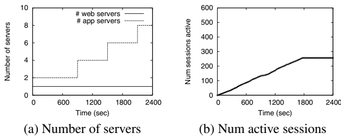
Figure 6. Rubbos: Provision only the Tomcat tier
