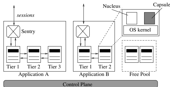
Figure 3. Hosting Platform Architecture.
