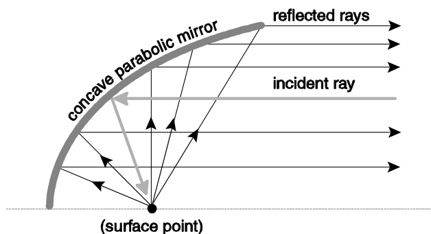
Figure 1: The focusing property of a concave parabolic mirror is exploited to simultaneously measure reflected rays from a large range of angles over the hemisphere. The same mirror is used to direct the incident illumination ray to the sample at the desired angle.
