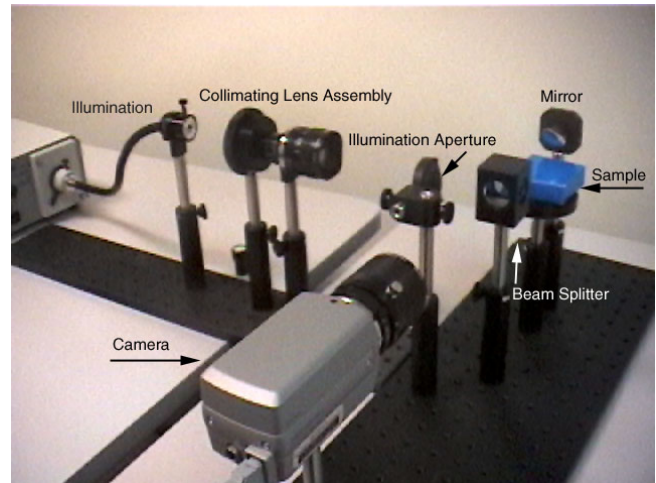
Figure 4: Device prototype including camera, illumination source, collimating lens assembly, illumination aperture, beam splitter and off-axis concave parabolic mirror. A blue specular sample to be measured is shown.
