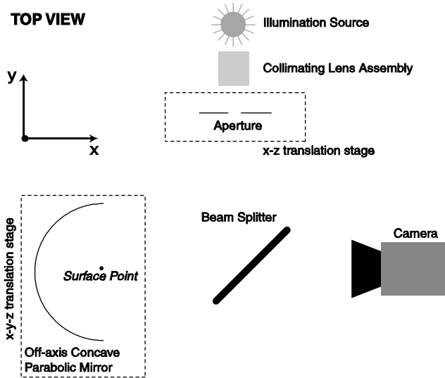
Figure 2: BRDF/BTF Measurement Device. The surface point is imaged by a CCD video camera observing an off-axis concave parabolic mirror to achieve simultaneous observation of a large range of viewing directions. Illumination direction is controlled by an aperture, i.e. translations of the aperture in the x - z plane cause variations in the illumination angle incident on the surface point. The device achieves illumination/viewing direction variations using a simple translations of the illumination aperture instead of complex gonioreflectometer equipment. Measurements of bidirectional texture are accomplished by translating the mirror in the x - y plane.
