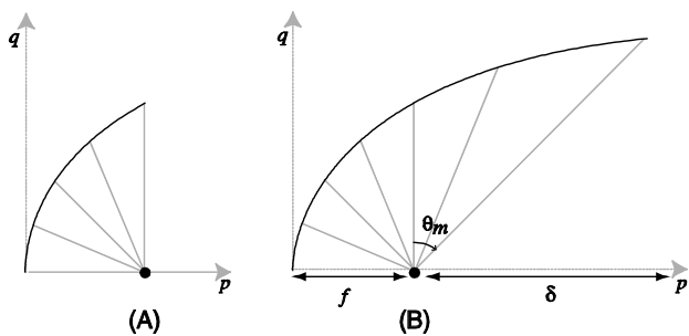
Figure 3: (A) Diagram of a typical concave parabolic mirror. (B) Diagram of an extended concave parabolic mirror.
