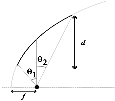
Figure 6: Cross-sectional view of mirror used in prototype. The focal point is a distance f from the vertex of the parabolic mirror and f = 12.7 mm. The mirror aperture is given by d = 25.4 mm. The angles defining the off-axis parabolic segment are \theta_1 = 36.5^\circ and \theta_2 = 22.8^\circ .
