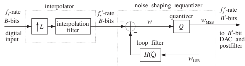
Fig. 12.7.6 Oversampled noise shaping requantizer for D/A conversion.
