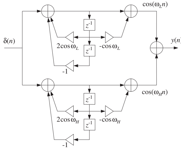
Fig. 8.1.4 DTMF tone generator.
