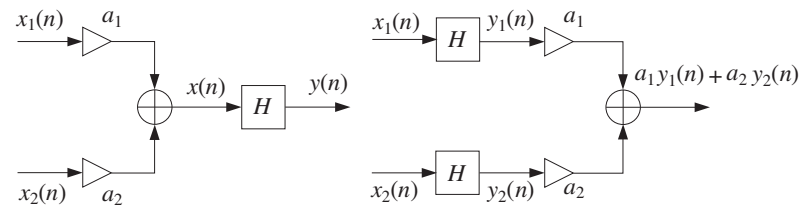
Fig. 3.2.1 Testing linearity.
