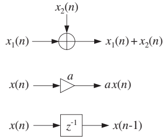
Fig. 4.2.1 Basic building blocks of DSP systems.
