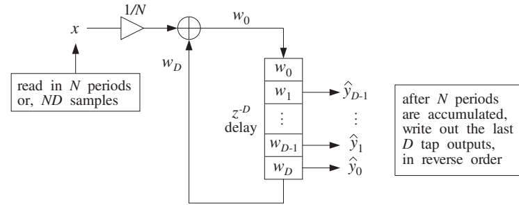
Fig. 8.3.28 Signal averaging implementation with a D -fold delay.
