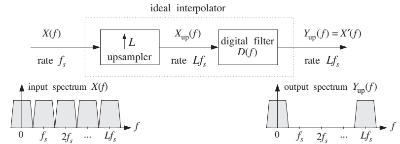
Fig. 12.2.6 Ideal interpolator in frequency domain.
