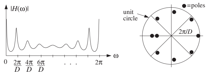
Fig. 8.2.24 Magnitude response of lowpass reverberator, for D = 8 .
