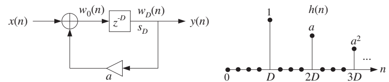
Fig. 8.2.26 Reverberating multi-delay.
