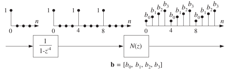
Fig. 8.1.9 Periodic pulse train causes periodic output.
