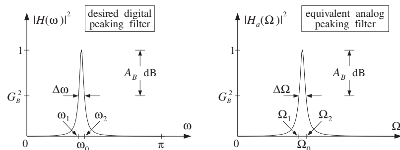
Fig. 11.3.2 Digital peaking filter and its analog equivalent.
