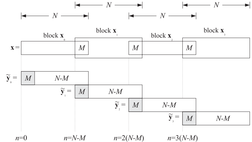
Fig. 9.9.1 Overlap-save method of fast convolution.
