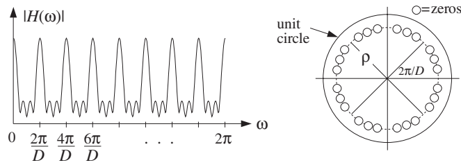
Fig. 8.2.5 Comb filter of Eq. (8.2.8), with peaks at \omega_k = 2\pi k/D, k = 0, 1, \dots, D - 1 .
