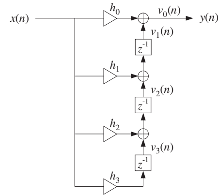
Fig. 4.3.1 Transposed realization of third-order filter.
