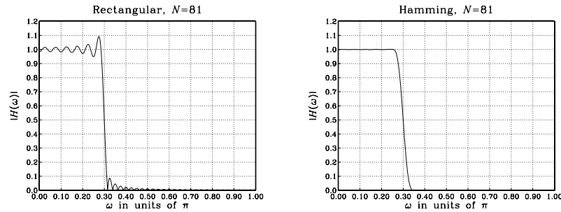
Fig. 10.1.7 Rectangular and Hamming windowed magnitude responses for N = 81 .
