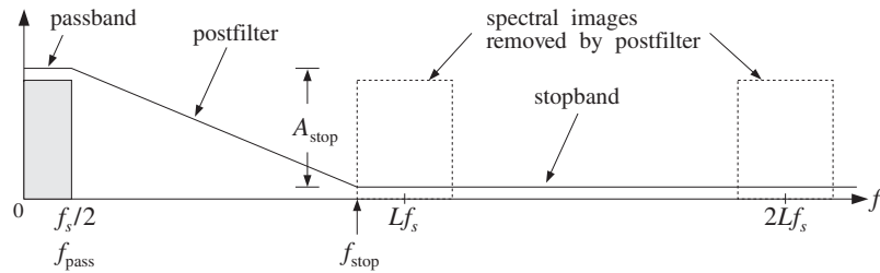
Fig. 12.4.20 Analog anti-image postfilter specifications.
