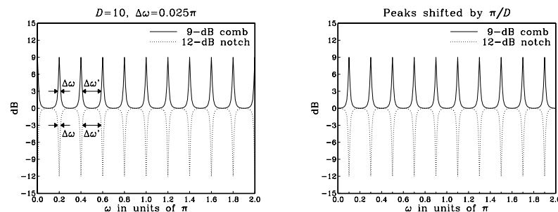
Fig. 11.5.1 Periodic peaking and notching comb filters.
