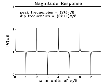
Fig. 7.4.3 Pole/zero sharpening in Example 7.4.4.
