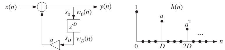
Fig. 8.2.6 Plain reverberator.
