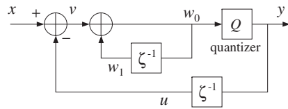
Fig. 12.8.2 Alternative model of first-order delta-sigma quantizer.
