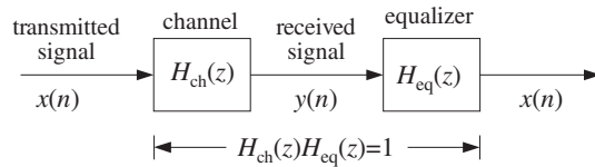
Fig. 6.5.2 Channel equalizer.
