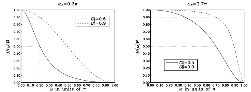
Fig. 11.2.3 First-order lowpass digital filters of Example 11.2.1.
