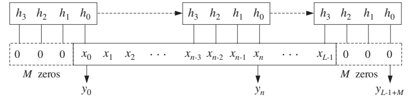
Fig. 4.1.4 Flip-and-slide form of convolution.
