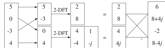
Fig. 9.8.6 4-point FFT of Example 9.8.1.
