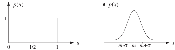
Fig. B.1 Uniform and Gaussian probability distributions.
