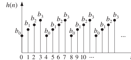
Fig. 8.1.6 Discrete-time periodic signal of period D = 4 .
