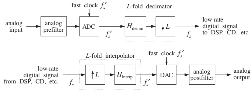
Fig. 12.5.5 Oversampling DSP system.
