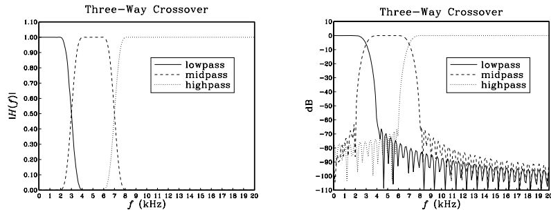
Fig. 10.2.8 Lowpass, midpass, and highpass magnitude responses.
