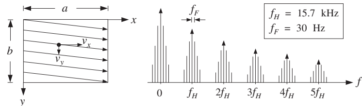
Fig. 8.3.20 Scanned image and corresponding video spectrum.
