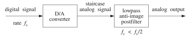
Fig. 12.1.4 Analog reconstruction of sampled signal.
