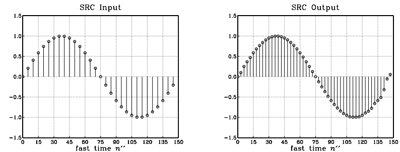
Fig. 12.8.1 Sample rate conversion by 5/3 .
