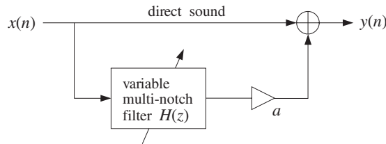
Fig. 8.2.12 Phasing effect with multi-notch filter.
