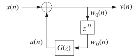
Fig. 8.2.20 Lowpass reverberator.
