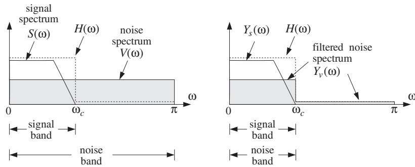
Fig. 8.3.2 Signal enhancement filter with partial noise reduction.
