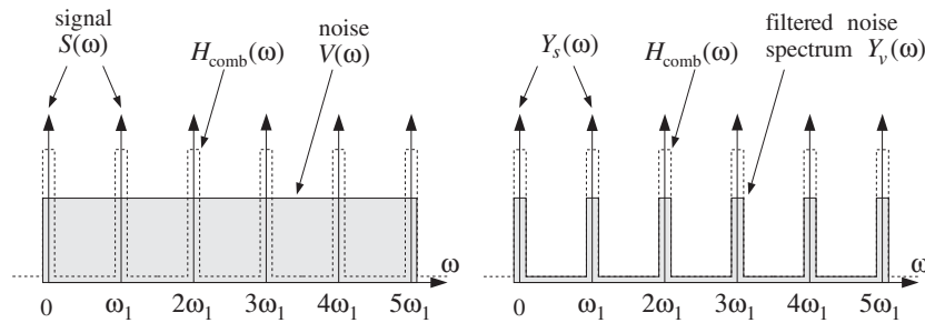
Fig. 8.3.11 Comb filter for enhancing periodic signal.
