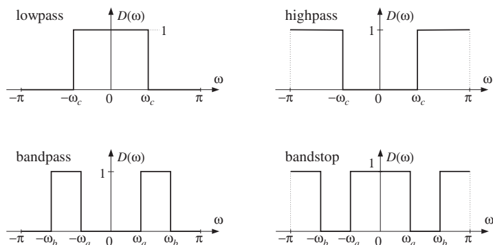
Fig. 10.1.1 Ideal lowpass, highpass, bandpass, and bandstop filters.
