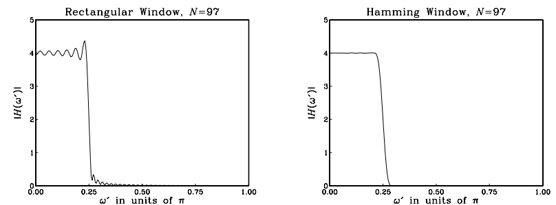
Fig. 12.4.8 Magnitude responses of length-97 interpolation filters.
