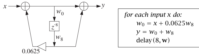
Fig. 7.4.2 Canonical realization of Example 7.4.3.
