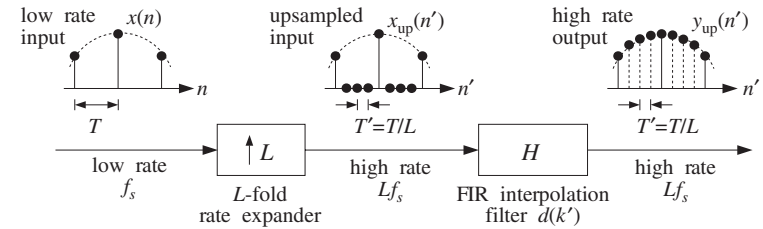
Fig. 12.2.1 L -fold digital interpolator.
