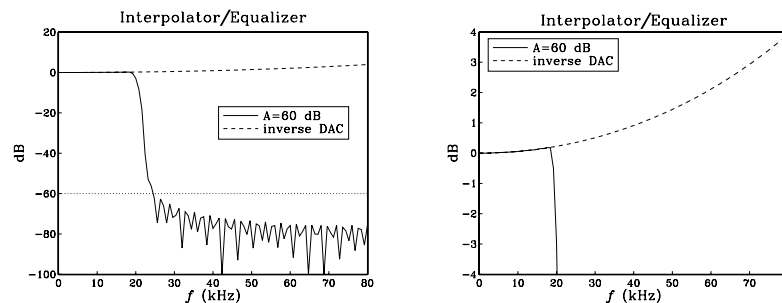
Fig. 12.4.18 4-fold interpolator/equalizer filter and its magnified passband.
