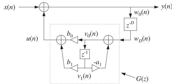
Fig. 8.2.21 Lowpass reverberator, with first-order feedback filter.
