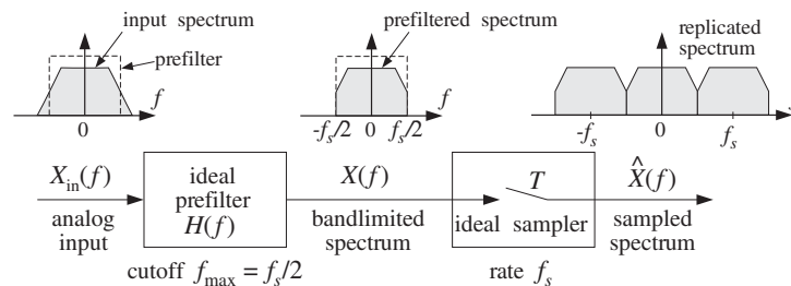
Fig. 1.5.5 Ideal antialiasing prefilter.
