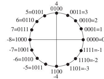
Fig. 2.3.2 Two's complement code.
