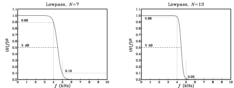
Fig. 11.6.3 Digital lowpass Butterworth filters.
