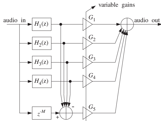
Fig. 10.2.11 Complementary implementation of graphic equalizer.
