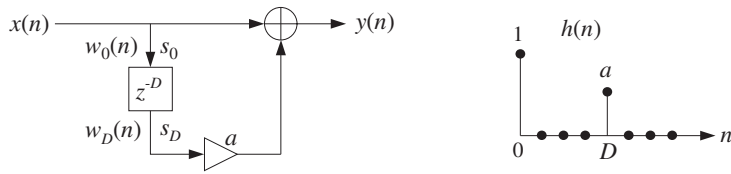
Fig. 8.2.2 Digital echo processor.
