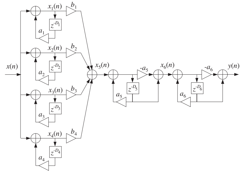
Fig. 8.2.18 Schroeder's reverb processor.
