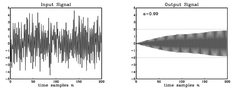
Fig. 8.3.6 Noisy input and high-frequency output for Example 8.3.2.
