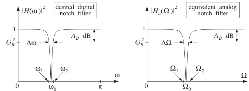
Fig. 11.3.1 Digital notch filter and its analog equivalent.
