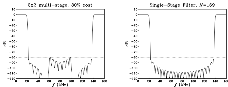
Fig. 12.4.14 Multistage filter H_0(f)H_1(f) and single-stage filter H(f) .
