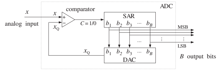
Fig. 2.4.2 Successive approximation A/D converter.
