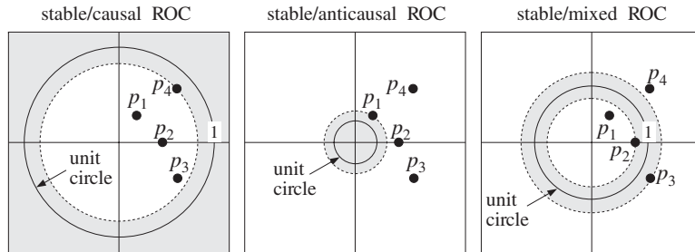
Fig. 5.3.2 Stable ROCs.
