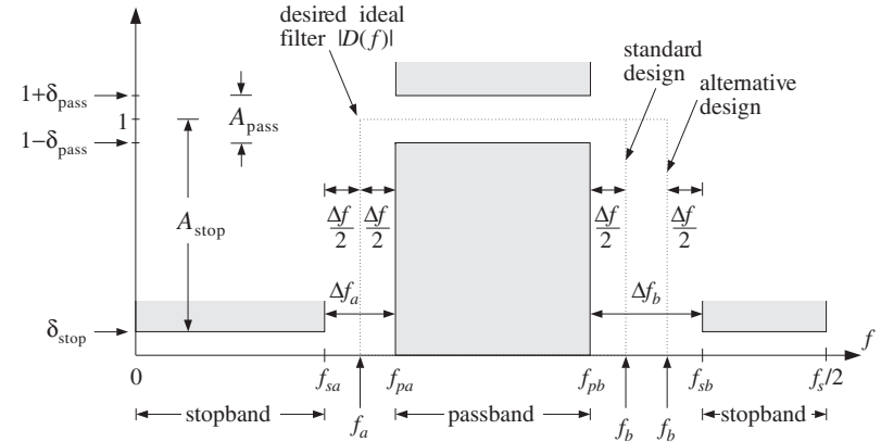
Fig. 10.2.3 Bandpass filter specifications.
