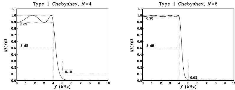
Fig. 11.6.11 Digital lowpass Chebyshev type 1 filters.
