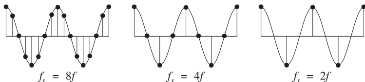
Fig. 1.4.1 Sinusoid sampled at rates f_s = 8f, 4f, 2f .
