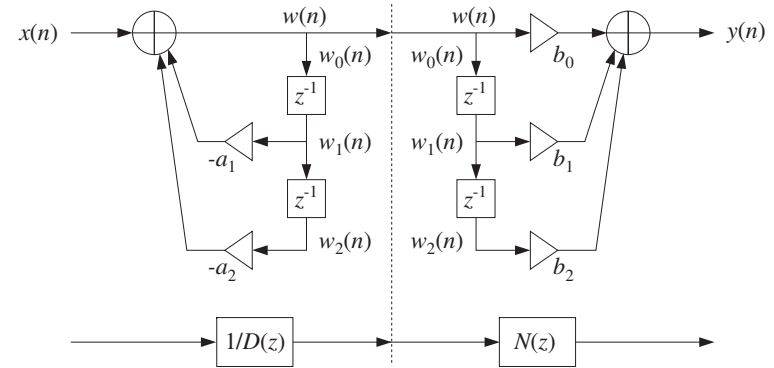
Fig. 7.2.2 Interchanging N(z) and 1/D(z) .
