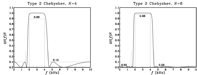
Fig. 11.6.14 Digital bandpass Chebyshev type 2 filters.
