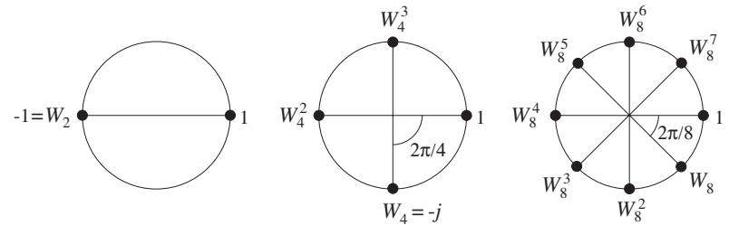
Fig. 9.4.1 Twiddle factor lookup tables for N = 2, 4, 8 .
