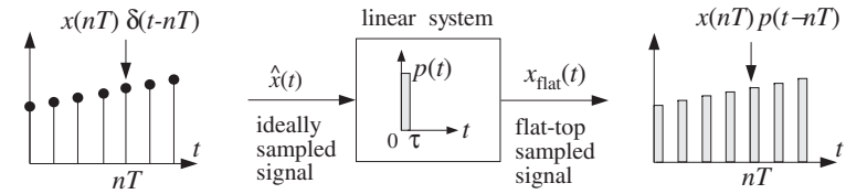
Fig. 1.8.2 Flat-top sampling as filtering.
