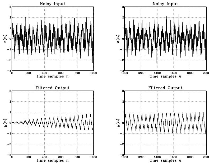
Fig. 8.3.19 Periodic signal enhancement by comb filtering.
