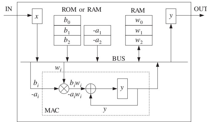
Fig. 7.5.1 Typical DSP chip realization of a second-order section.
