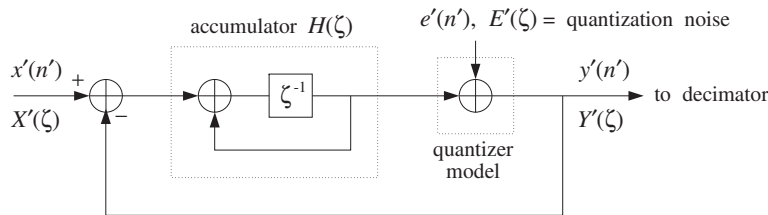
Fig. 12.7.2 Discrete-time model of first-order delta-sigma quantizer.
