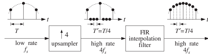
Fig. 12.1.1 Sampling rate increase with digital interpolation.
