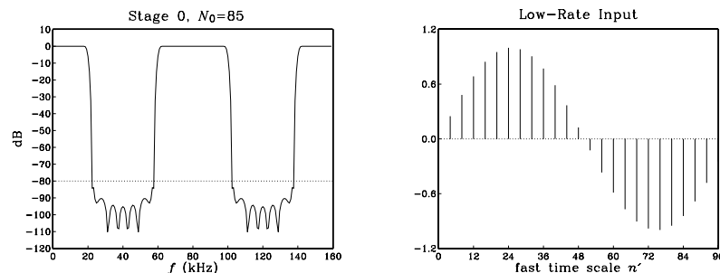
Fig. 12.4.11 Filter H_0(f) and its low-rate input signal.
