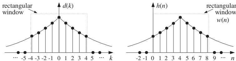
Fig. 10.1.3 Rectangularly windowed impulse response, with N = 9 , M = 4 .
