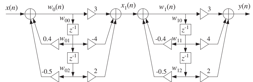
Fig. 7.3.2 Cascade realization of Example 7.3.1.
