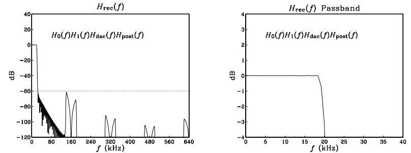
Fig. 12.4.27 Effective reconstructor has flat passband and 60 dB stopband.
