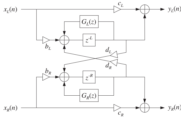
Fig. 8.4.1 Stereo delay effects processor.
