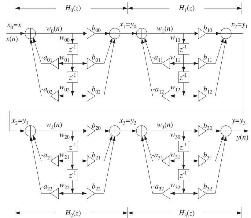
Fig. 7.3.1 Cascade of second-order sections.
