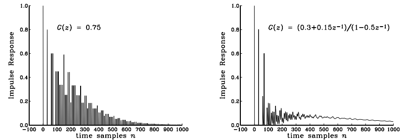
Fig. 8.2.28 Impulse response of plain and lowpass multi-delay.
