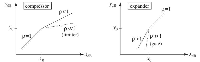
Fig. 8.2.31 Input/output relationship of compressor or expander.
