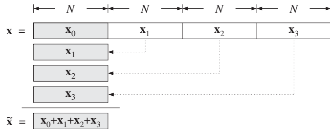
Fig. 9.5.1 Modulo-N reduction of a signal.
