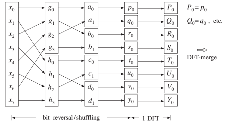
Fig. 9.8.3 Shuffling process generates N 1-dimensional signals.
