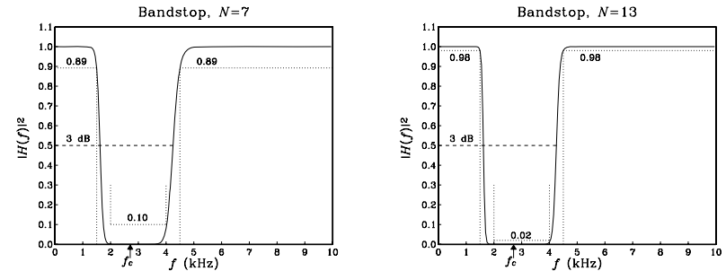
Fig. 11.6.9 Digital bandstop Butterworth filters.
