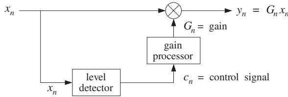
Fig. 8.2.32 Compressor/expander dynamics processor.
