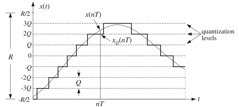
Fig. 2.1.2 Signal quantization.
