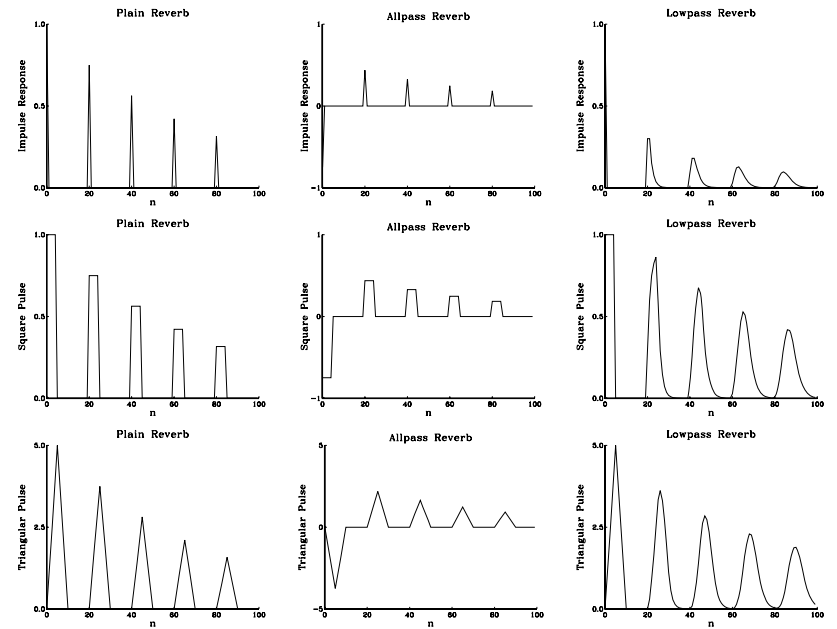
Fig. 8.2.22 Comparison of plain, allpass, and lowpass reverberators.
