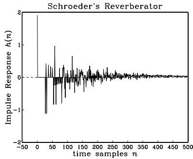
Fig. 8.2.19 Impulse response of Schroeder's reverberator.
