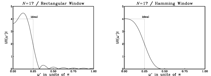
Fig. 12.4.4 Magnitude response |H(\omega')| versus \omega' = 2\pi f/f_s' .
