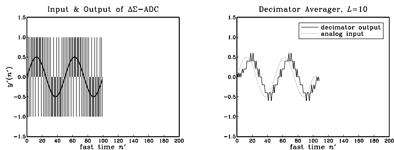
Fig. 12.7.4 Delta-sigma quantizer output and averaging decimator's output.
