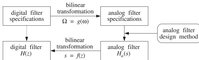
Fig. 11.1.1 Bilinear transformation method.
