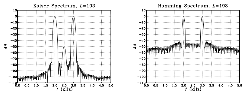
Fig. 10.2.12 Kaiser and Hamming spectra.
