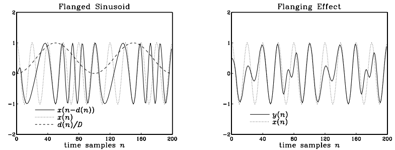
Fig. 8.2.9 Flanged sinusoidal signal.
