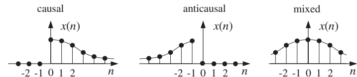
Fig. 3.5.1 Causal, anticausal, and mixed signals.
