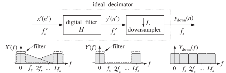
Fig. 12.5.3 Ideal digital decimator in frequency domain.
