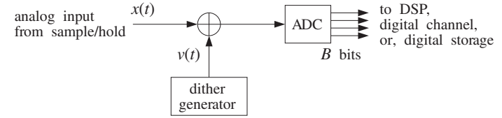
Fig. 2.5.1 Analog dither.
