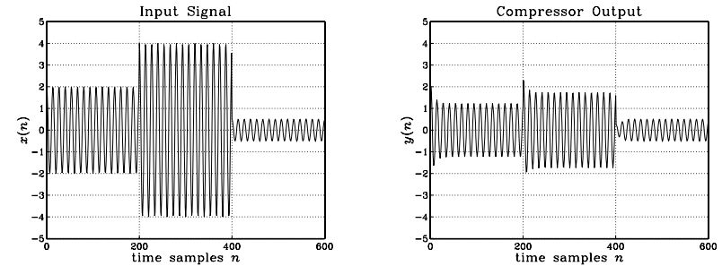
Fig. 8.2.33 Compressor input and output signals ( \rho = 1/2 , \lambda = 0.9 , c_0 = 0.5 ).
