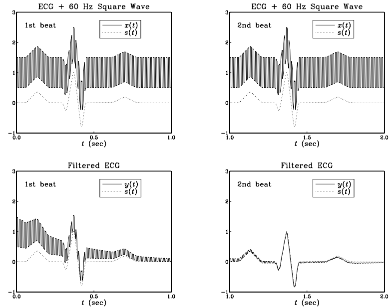
Fig. 8.3.14 Eliminating baseline shifts and 60 Hz harmonics from ECG.
