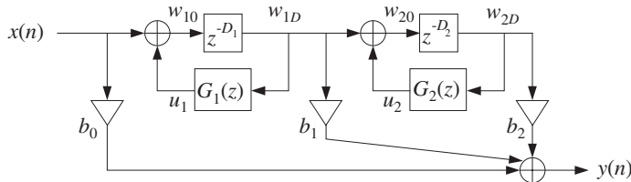
Fig. 8.2.27 Multi-delay effects processor.
