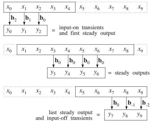
Fig. 8.3.32 Steady-state and transient outputs for L = 10, N = 5 .
