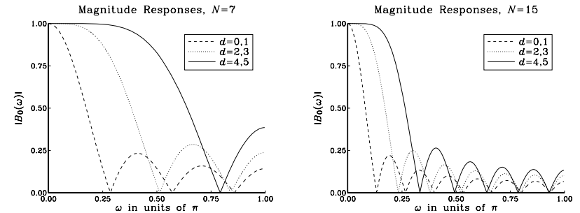
Fig. 8.3.31 Savitzky-Golay filters of lengths N = 7, 15 , and orders d = 0, 2, 4 .
