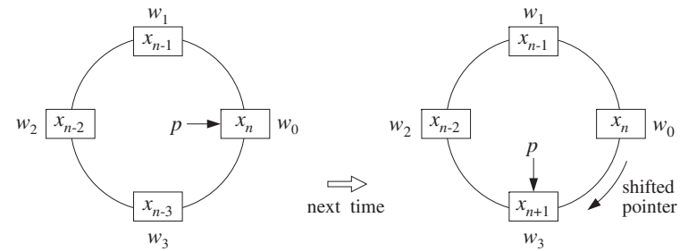
Fig. 4.2.12 Modulo- (M+1) circular delay-line buffer.
