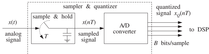
Fig. 2.1.1 Analog to digital conversion.
