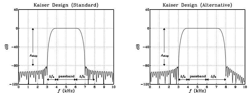
Fig. 10.2.5 Kaiser window design of a bandpass filter.
