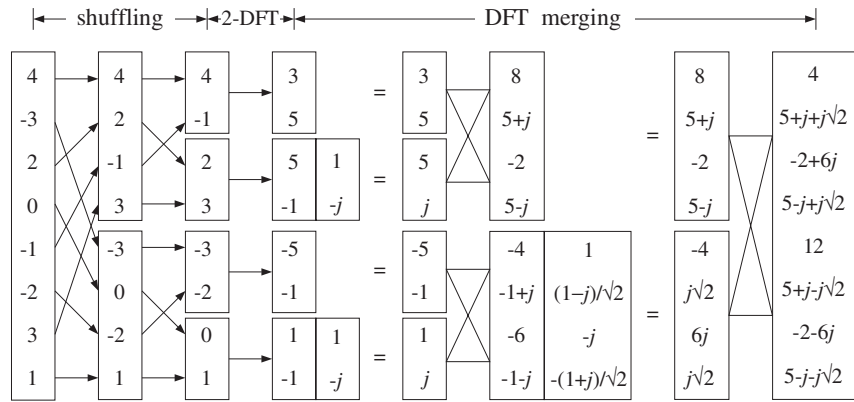
Fig. 9.8.7 8-point FFT of Example 9.8.2.
