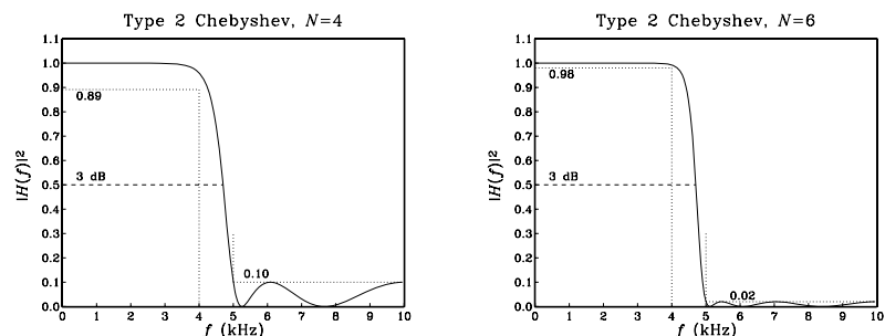
Fig. 11.6.13 Digital lowpass Chebyshev type 2 filters.
