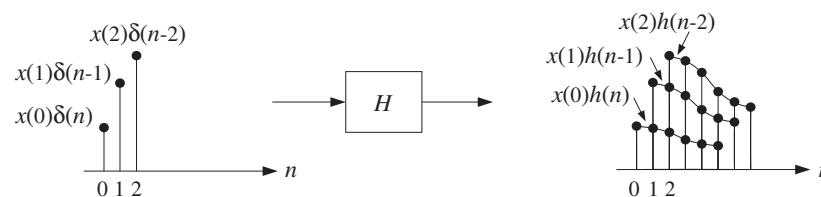
Fig. 3.3.3 Response to linear combination of inputs.
