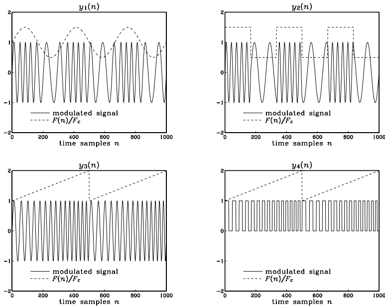
Fig. 8.1.23 Frequency modulated waveforms.
