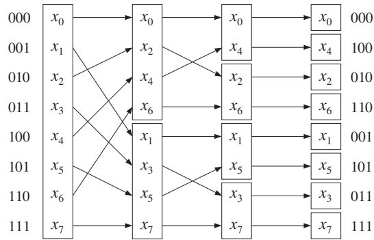
Fig. 9.8.5 Shuffling is equivalent to bit reversal.
