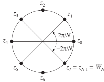
Fig. 9.2.3 N th roots of unity, for N = 8 .
