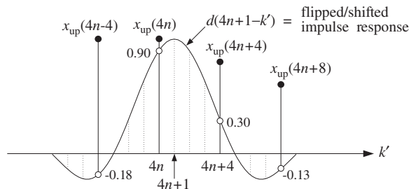
Fig. 12.4.3 Flip-and-slide form of convolution.
