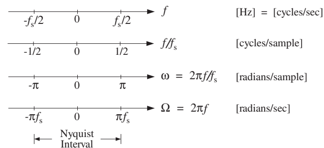
Fig. 1.4.4 Commonly used frequency units.
