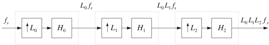
Fig. 12.2.8 Three-stage interpolation filter.
