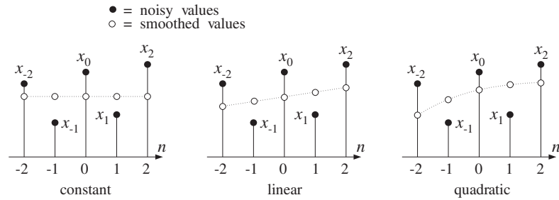
Fig. 8.3.30 Data smoothing with polynomials of degrees d = 0, 1, 2 .
