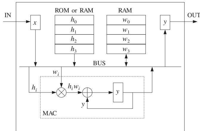
Fig. 4.2.10 Typical DSP chip.
