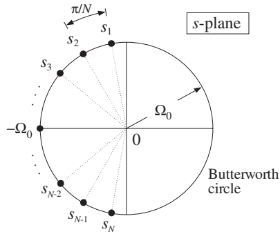
Fig. 11.6.2 Butterworth filter poles lie on Butterworth circle.
