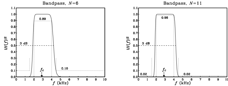
Fig. 11.6.7 Digital bandpass Butterworth filters.
