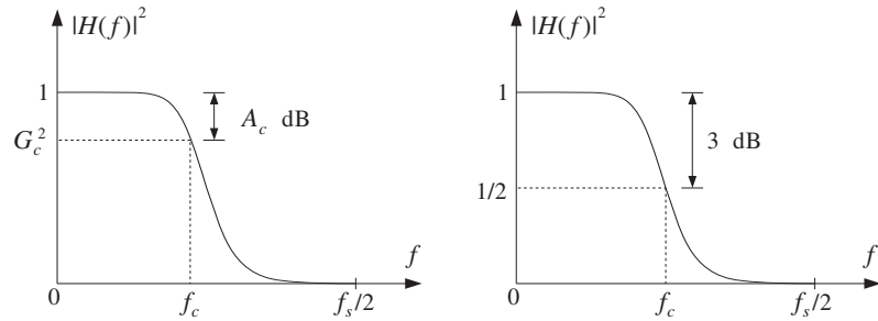
Fig. 11.2.1 Cutoff frequency specifications for lowpass digital filter.
