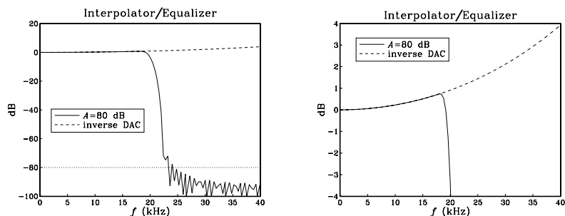
Fig. 12.4.16 2-fold interpolator/equalizer designed with A = 80 dB.
