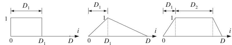
Fig. 8.1.17 Square, triangular, and trapezoidal waveforms.
