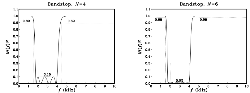
Fig. 11.6.15 Digital bandstop Chebyshev type 2 filters.
