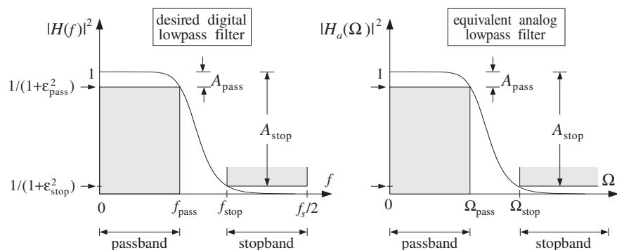
Fig. 11.6.1 Lowpass digital filter and its analog equivalent.
