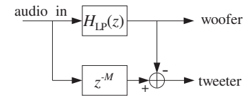
Fig. 10.2.7 Complementary implementation of two-way crossover filters.
