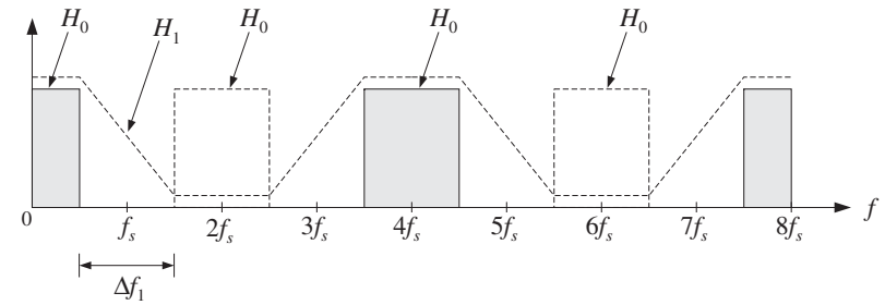
Fig. 12.2.9 Two-stage 2 \times 2 interpolation filter.
