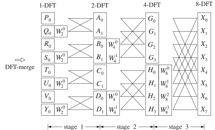
Fig. 9.8.4 DFT merging.
