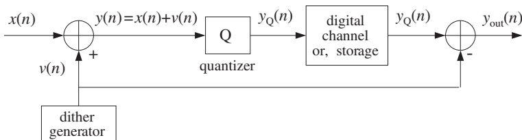
Fig. 2.5.4 Subtractive dither.
