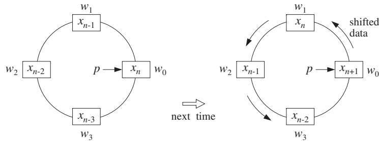
Fig. 4.2.11 Wrapped linear delay-line buffer.
