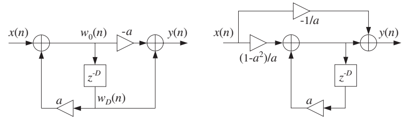
Fig. 8.2.17 Allpass reverberator in canonical and parallel form.
