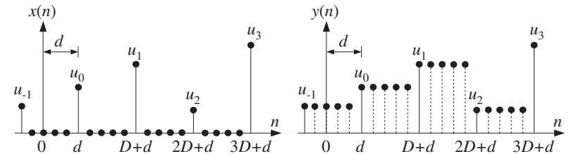
Fig. B.6 Randomly delayed input and output sequences.
