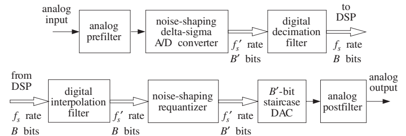
Fig. 2.2.5 Oversampling DSP system.
