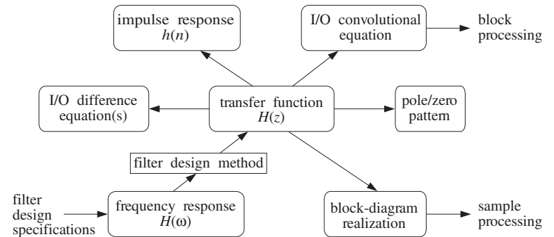
Fig. 6.1.1 Equivalent descriptions of digital filters.
