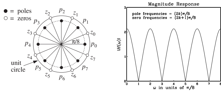
Fig. 7.4.1 Pole/zero pattern and magnitude response of Example 7.4.3.
