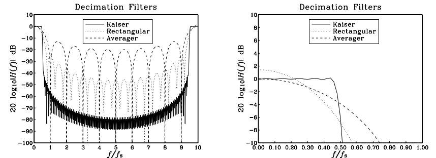
Fig. 12.7.3 Magnitude responses of decimation filters.
