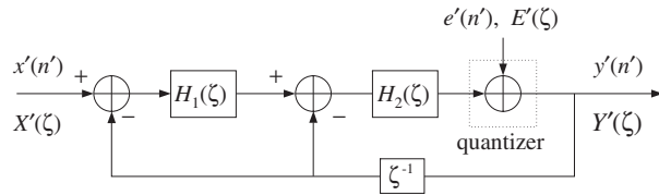
Fig. 12.8.3 Discrete-time model of second-order delta-sigma quantizer.
