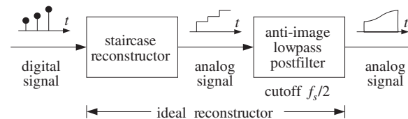
Fig. 1.6.7 Analog anti-image postfilter.
