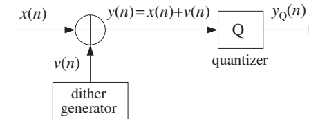
Fig. 2.5.2 Nonsubtractive dither process and quantization.
