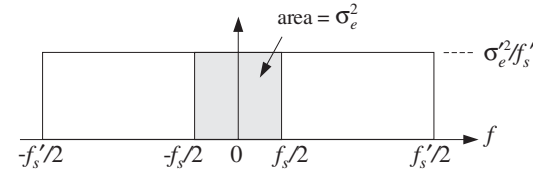
Fig. 2.2.3 Oversampled quantization noise power, without noise shaping.
