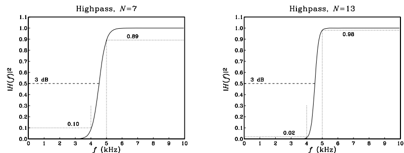
Fig. 11.6.5 Digital highpass Butterworth filters.
