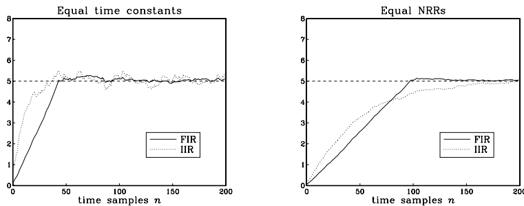
Fig. 8.3.7 Comparison of FIR and IIR smoothing filters.
