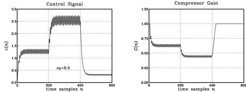
Fig. 8.2.34 Compressor control signal and gain ( \rho = 1/2 , \lambda = 0.9 , c_0 = 0.5 ).
