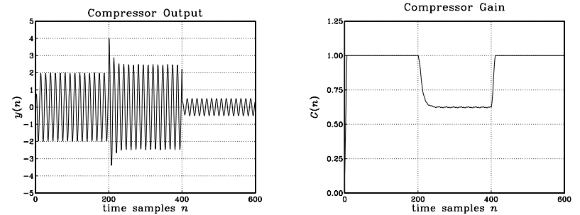
Fig. 8.2.36 Limiter output with smoothed gain ( \rho = 1/10 , \lambda = 0.9 , c_0 = 1.5 ).
