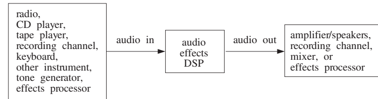
Fig. 8.2.1 Audio effects signal processor.
