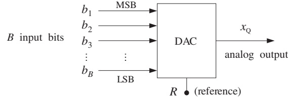
Fig. 2.3.1 B -bit D/A converter.
