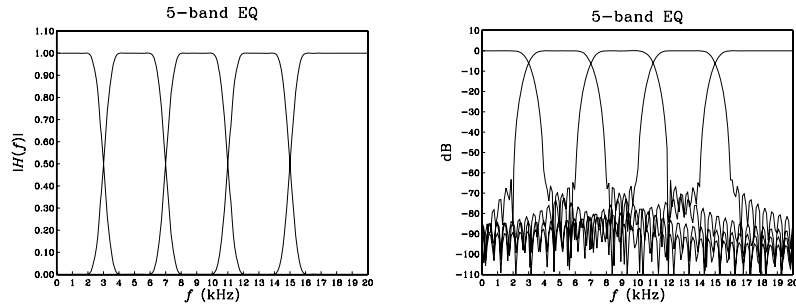
Fig. 10.2.10 Graphic equalizer magnitude responses.
