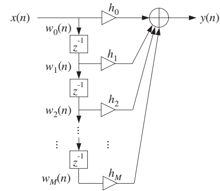
Fig. 4.2.9 Direct form realization of M th order filter.
