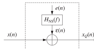
Fig. 2.2.2 Model of noise shaping quantizer.
