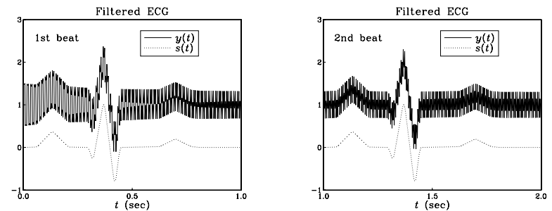
Fig. 8.3.15 Inadequate filtering by the single-notch filter H_1(z) .
