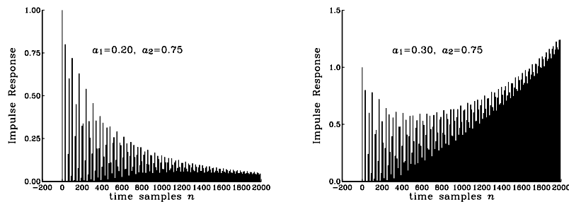
Fig. 8.2.30 Impulse response of multi-tap delay line.
