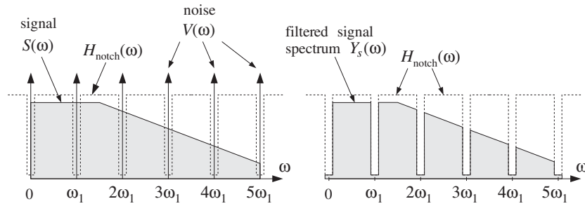
Fig. 8.3.10 Notch filter for reducing periodic interference.
