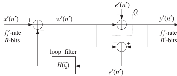
Fig. 12.7.7 Noise shaping requantizer model.
