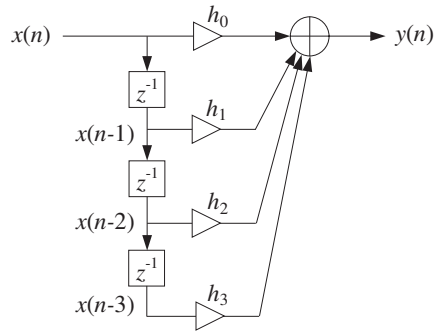
Fig. 4.2.6 Direct form realization of third-order filter.
