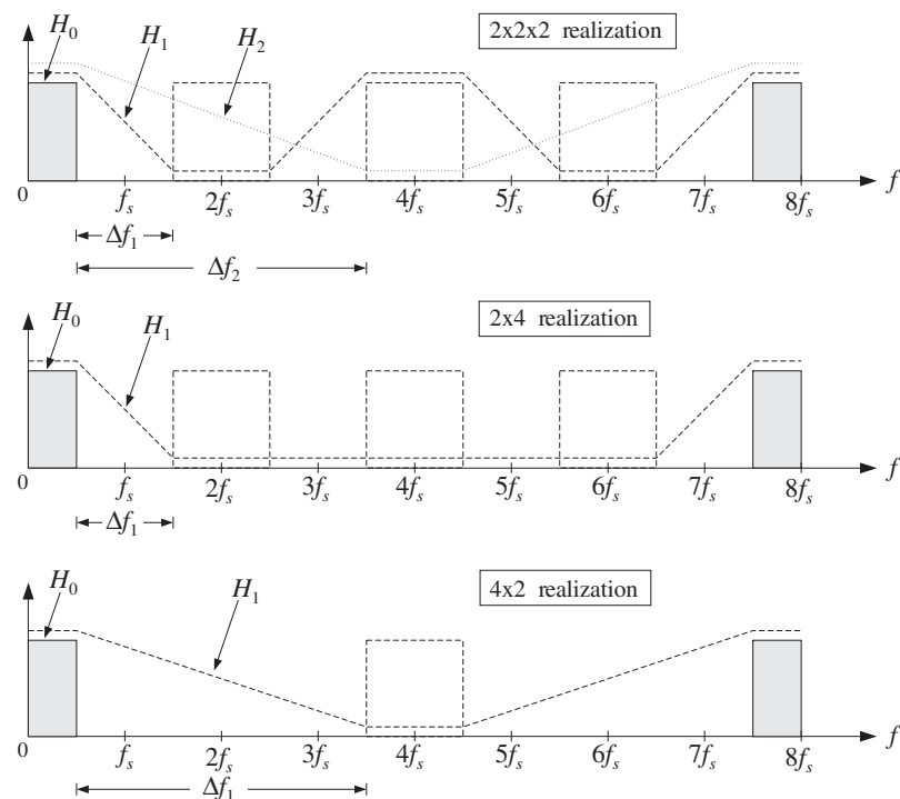
Fig. 12.2.10 Frequency characteristics of multistage 8-fold interpolators.
