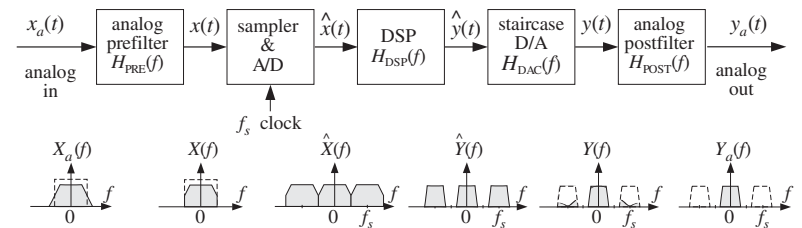
Fig. 1.7.1 Components of typical DSP system.
