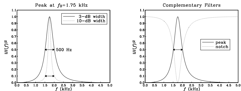
Fig. 11.3.3 Peaking and complementary notch filters.
