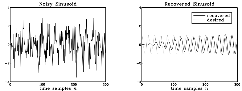
Fig. 8.3.9 Noisy sinusoidal input and extracted sinusoid.
