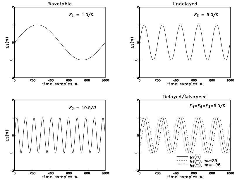
Fig. 8.1.18 Waveforms generated from a common wavetable.
