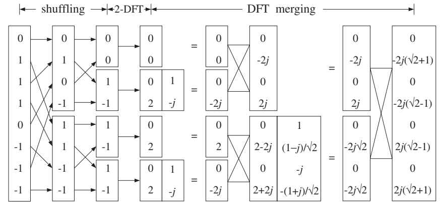
Fig. 9.8.9 8-point FFT of the square wave in Example 9.8.3.
