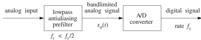
Fig. 12.1.2 Prefiltering and sampling of analog signal.
