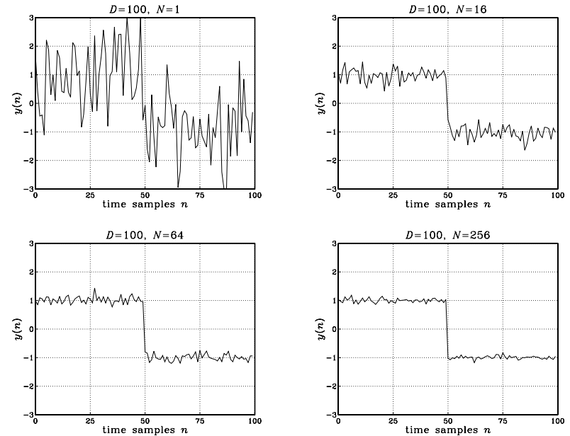
Fig. 8.3.29 Signal averaging with D = 100 , and N = 1, 16, 64, 256 sweeps.
