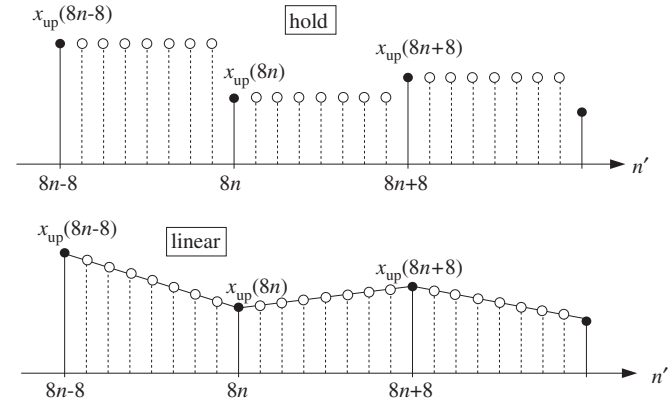
Fig. 12.3.2 8-fold hold and linear interpolators.
