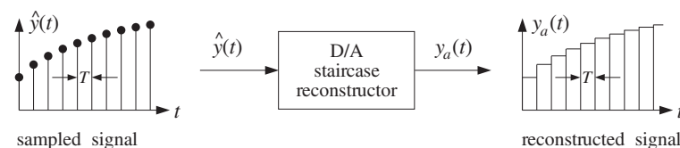
Fig. 1.6.1 Staircase reconstructor.
