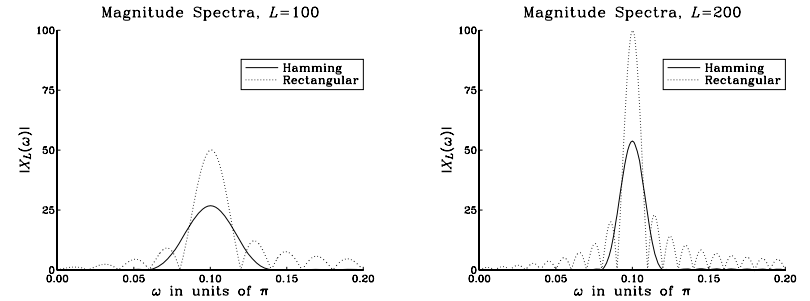
Fig. 9.1.7 Rectangular and Hamming spectra for L = 100 and L = 200 .
