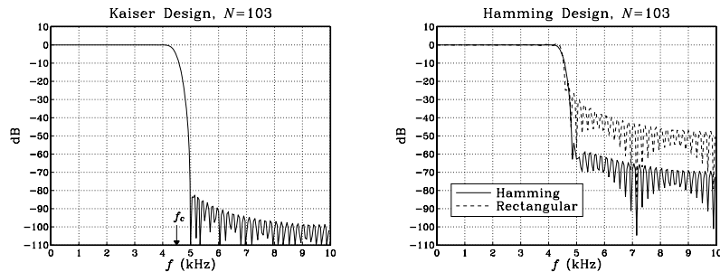
Fig. 10.2.4 Kaiser, Hamming, and rectangular window designs, N = 103 .
