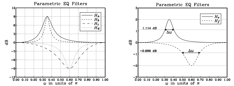
Fig. 11.4.2 Parametric EQ filters of Example 11.4.1.
