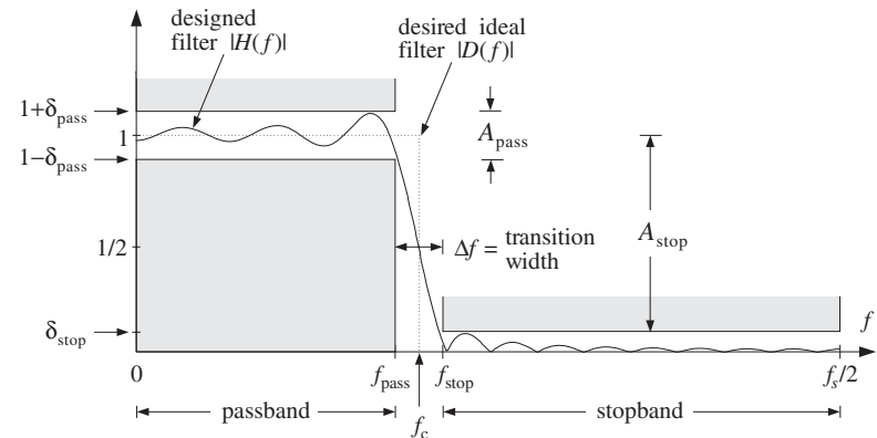
Fig. 10.2.1 Magnitude response specifications for a lowpass filter.
