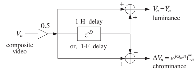
Fig. 8.3.22 Line or frame comb filters.
