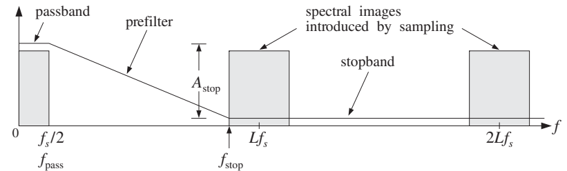
Fig. 12.5.4 Analog prefilter specifications for L -fold decimation.
