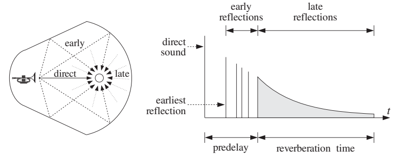
Fig. 8.2.15 Reverberation impulse response of a listening space.
