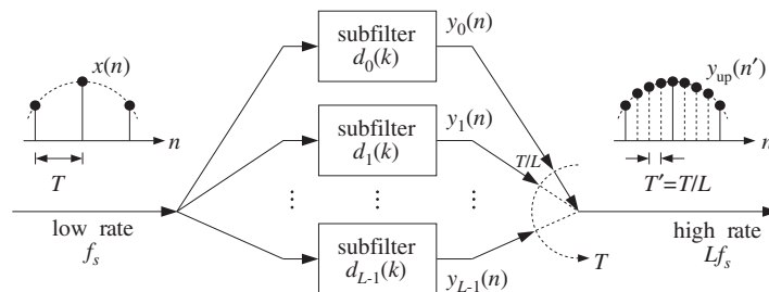
Fig. 12.2.5 Polyphase subfilter implementation of digital interpolator.
