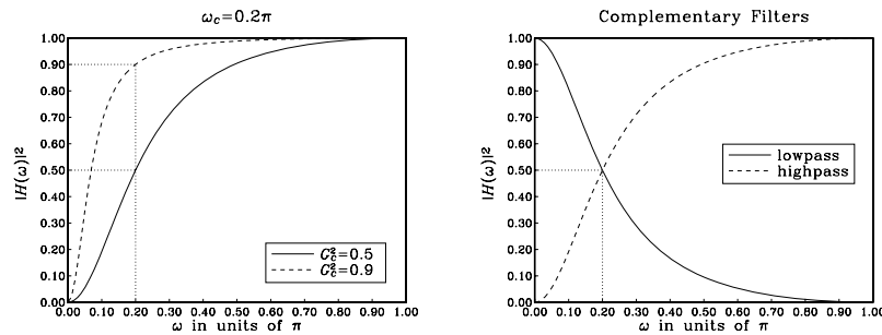
Fig. 11.2.5 Highpass and complementary lowpass digital filters.
