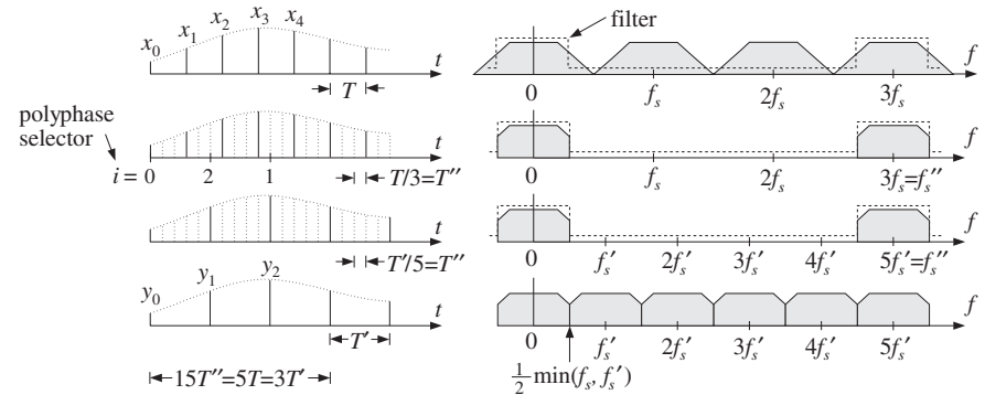
Fig. 12.6.3 Sampling rate conversion by a factor of 3/5 .
