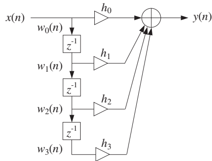
Fig. 4.2.7 Direct form with internal states.
