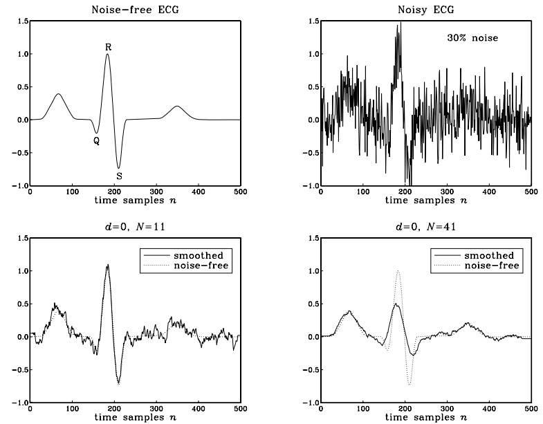
Fig. 8.3.33 Savitzky-Golay filter comparisons, for N = 11, 41 and d = 0 .
