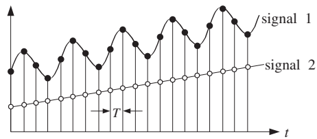
Fig. 1.3.3 Signal 2 is oversampled.
