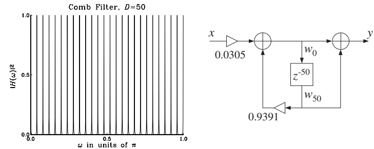
Fig. 8.3.18 Comb filter with D = 50 and Q = 50 .
