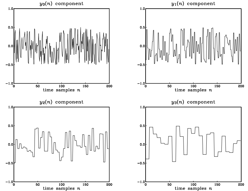
Fig. B.8 Components of 1/f noise.
