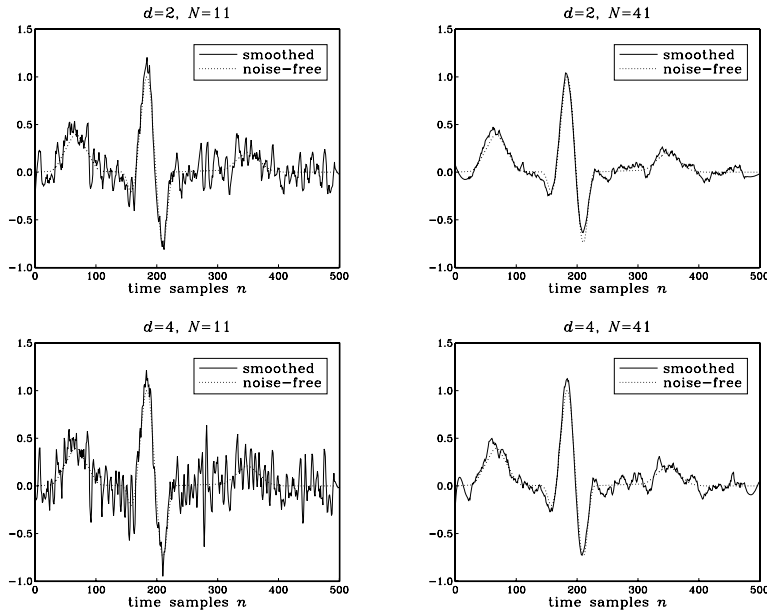
Fig. 8.3.34 Savitzky-Golay filter comparisons, for N = 11, 41 and d = 2, 4 .
