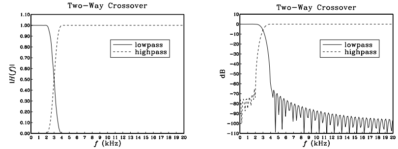
Fig. 10.2.6 Low- and high-frequency magnitude responses.
