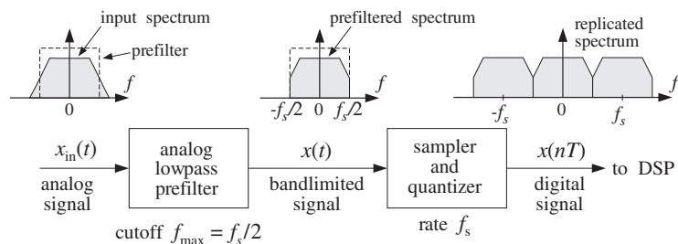
Fig. 1.3.5 Antialiasing prefilter.
