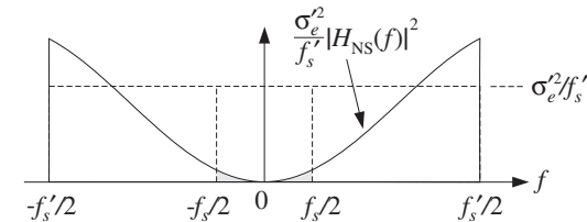
Fig. 2.2.4 Spectrum of oversampling noise shaping quantizer.
