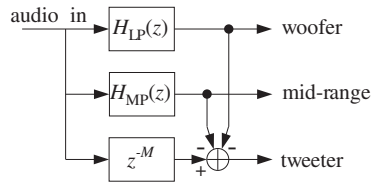
Fig. 10.2.9 Complementary implementation of three-way crossover filters.
