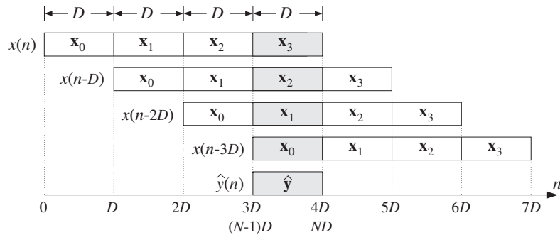
Fig. 8.3.27 Signal averaging as FIR comb filtering.
