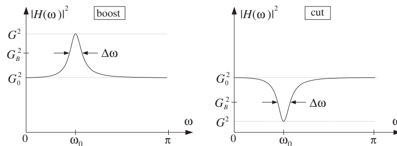
Fig. 11.4.1 Parametric EQ filter with boost or cut.
