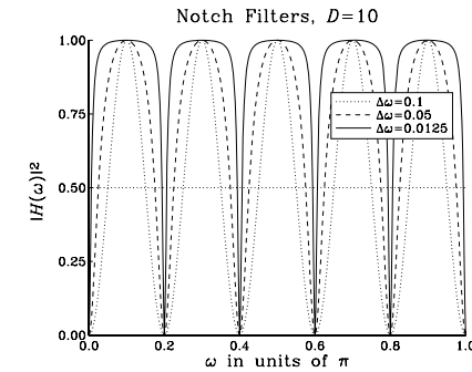
Fig. 8.3.13 Multi-notch filters of different widths ( \Delta\omega in units of \pi ).
