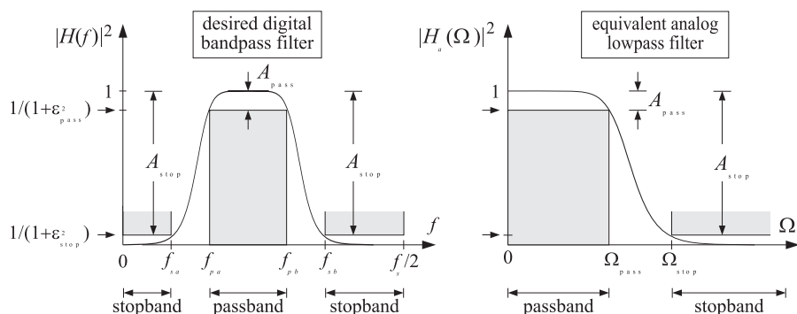
Fig. 11.6.6 Bandpass digital filter and its analog lowpass equivalent.
