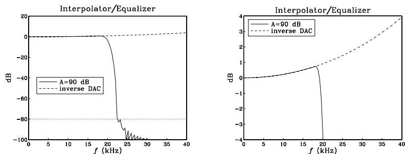
Fig. 12.4.17 2-fold interpolator/equalizer redesigned with A = 90 dB.
