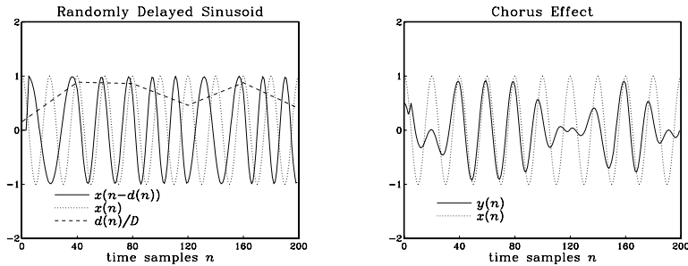
Fig. 8.2.11 Chorusing or doubling of sinusoidal signal.
