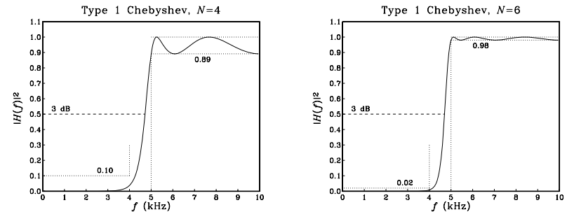
Fig. 11.6.12 Digital highpass Chebyshev type 1 filters.
