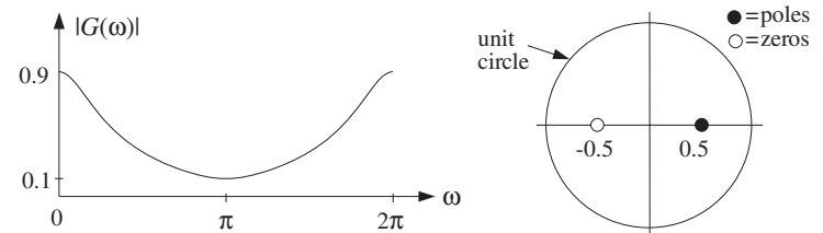
Fig. 8.2.23 Magnitude response of lowpass feedback filter G(z) .
