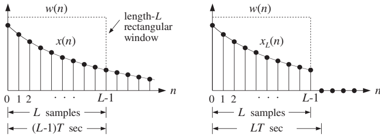
Fig. 9.1.1 Time windowing.
