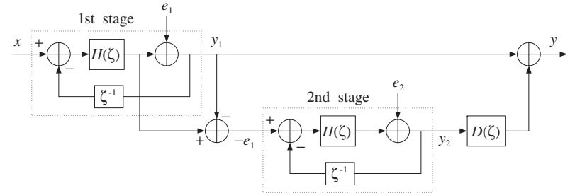
Fig. 12.8.4 MASH architecture of second-order delta-sigma quantizer.
