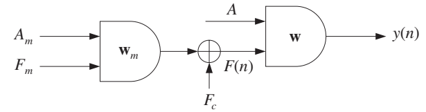
Fig. 8.1.22 Frequency modulation.
