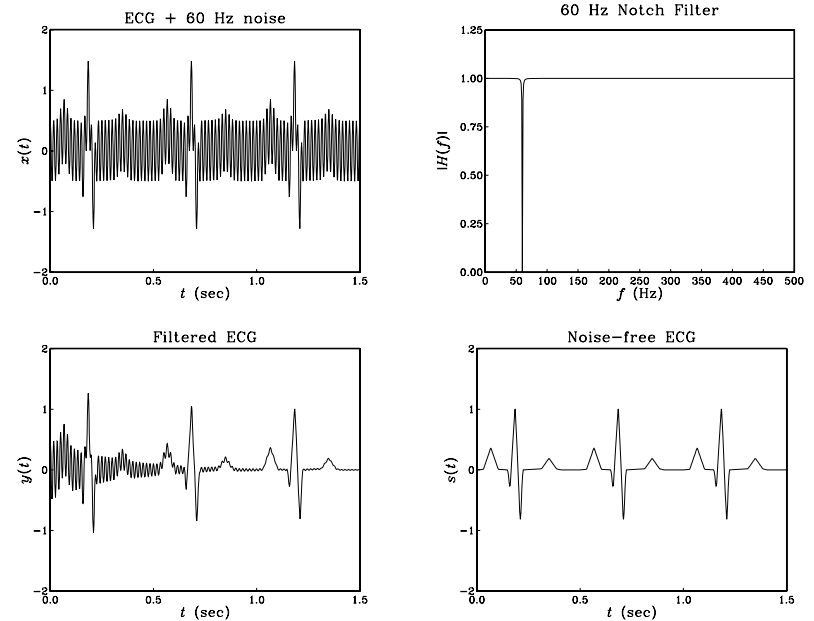
Fig. 8.3.12 Removing 60 Hz noise from ECG signal.
