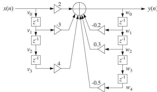
Fig. 7.1.3 Direct form realization of Example 7.1.1.
