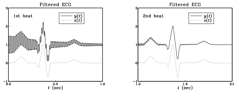
Fig. 8.3.16 Output from the cascade filter H_1(z)H_3(z)H_5(z) .
