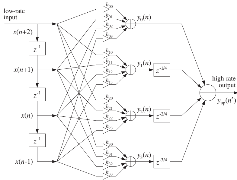
Fig. 12.4.5 Polyphase realization of 4-fold interpolator.
