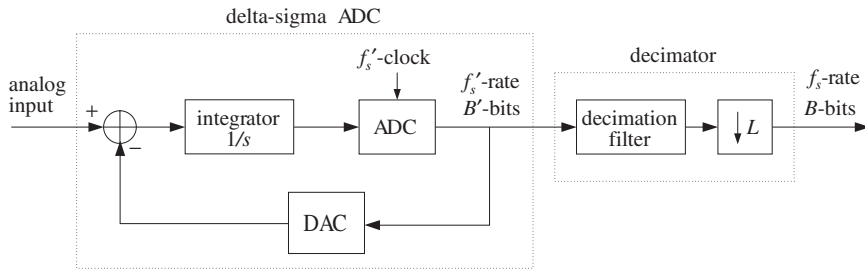
Fig. 12.7.1 Oversampled first-order delta-sigma A/D converter.
