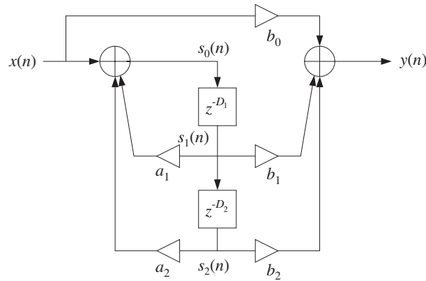
Fig. 8.2.29 Multitap delay effects processor.
