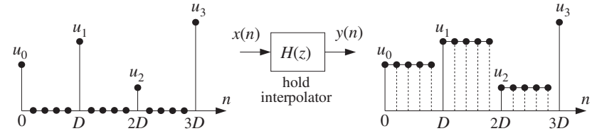
Fig. B.5 Filtering interpretation of hold interpolator.
