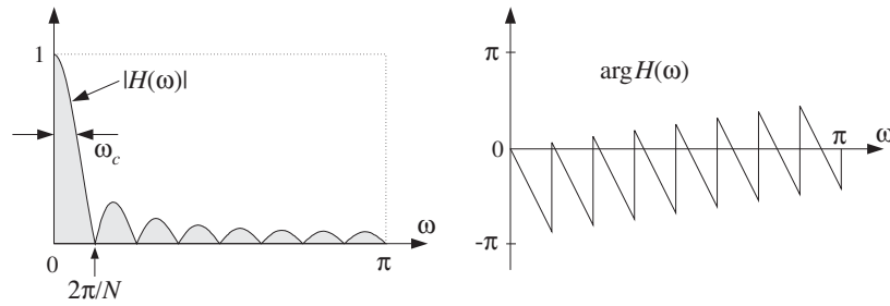
Fig. 8.3.8 Magnitude and phase responses of FIR smoother, for N = 16 .
