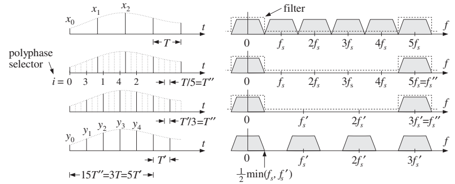
Fig. 12.6.2 Sampling rate conversion by a factor of 5/3.
