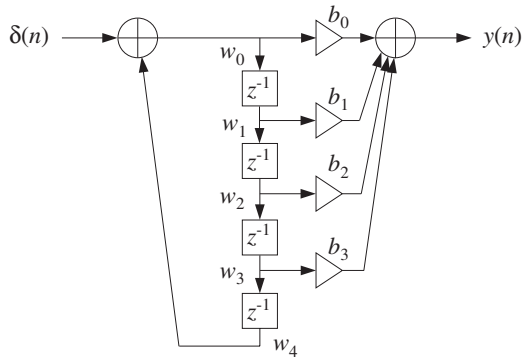
Fig. 8.1.8 Periodic generator in canonical form.
