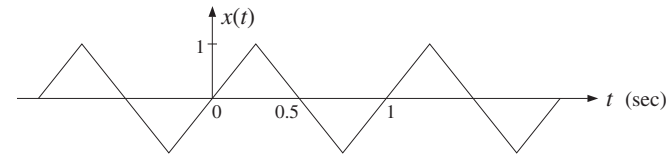
Fig. 1.8.1 Triangular waveform of Problem 1.7.
