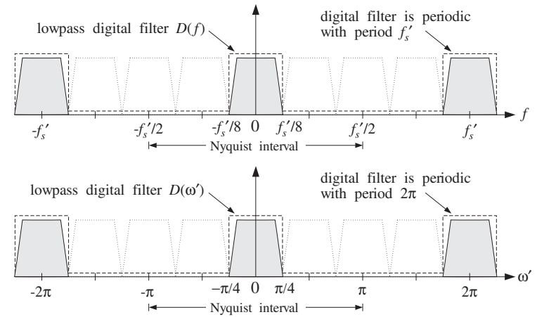
Fig. 12.1.9 High-rate FIR interpolator removes intermediate spectral images.
