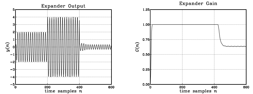
Fig. 8.2.37 Expander output and gain ( \rho = 2 , \lambda = 0.9 , c_0 = 0.5 ).
