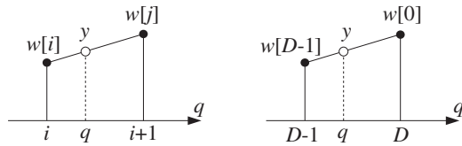
Fig. 8.1.13 Linear interpolation between two successive buffer samples.
