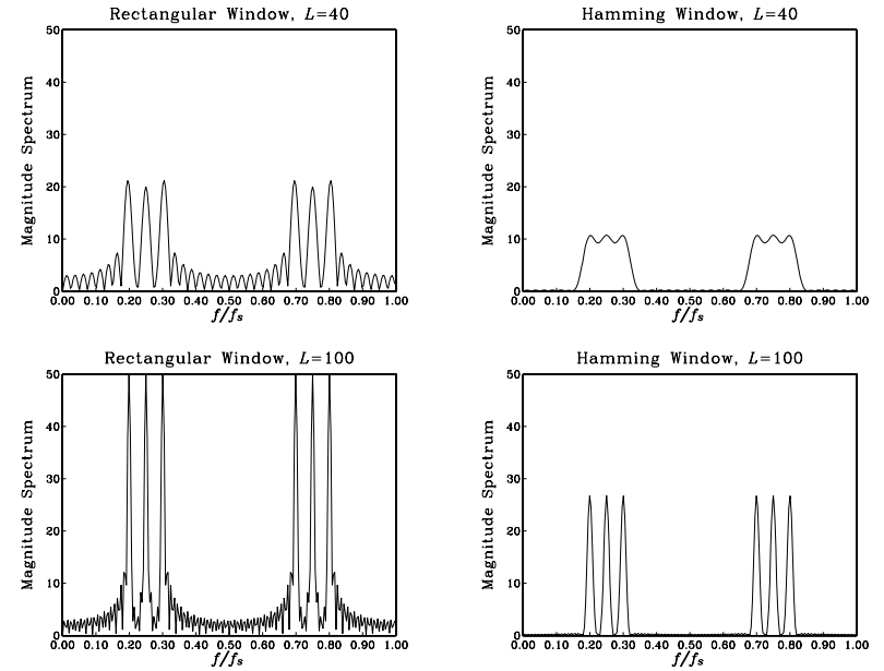
Fig. 9.1.9 Rectangular and Hamming spectra for L = 40 and 100 .
