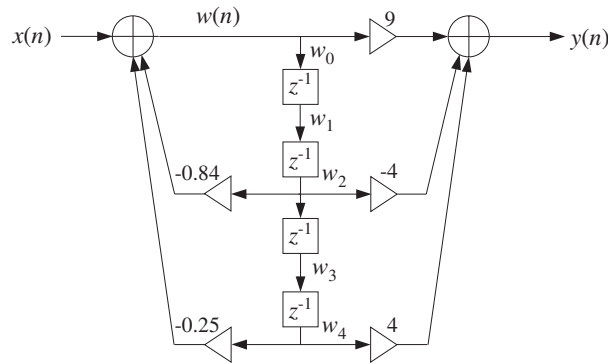
Fig. 7.3.3 Canonical realization of Example 7.3.1.
