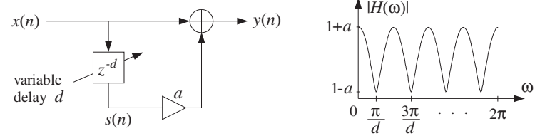
Fig. 8.2.8 Flanging effect, created with a periodically varying delay d(n) .
