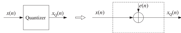
Fig. 2.1.3 Additive noise model of a quantizer.
