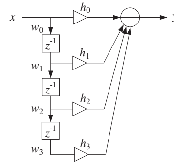
Fig. 4.2.8 Block diagram form of sample processing algorithm.
