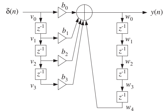
Fig. 8.1.7 Periodic generator in direct form.
