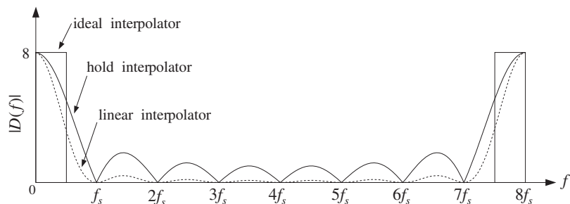
Fig. 12.3.3 Hold and linear interpolator frequency responses for L = 8 .
